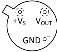
NDV Package 3-Pin TO-CAN (Top View)
